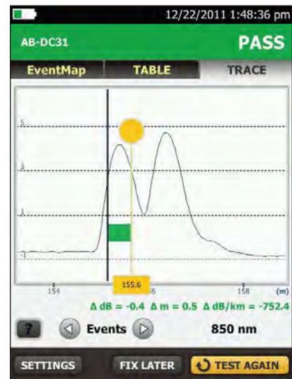
Extremely short event and attenuation dead zone
